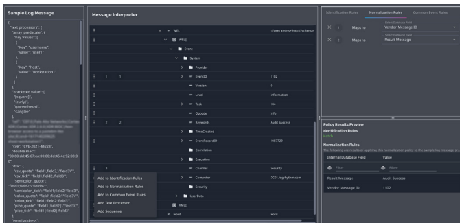
Figure 3: Easily parse unidentified logs with LogRhythm Policy Builder feature.
